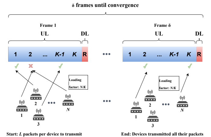
Figure 2. Frame in UL and DL time-slots until the end of system transmission (all devices), namely convergence of transmission process.
