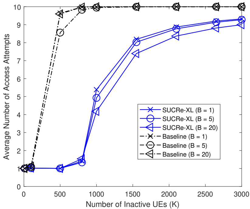
Figure 3.2 – Average number of access attempts vs. number of inactive UEs, corroborating the better performance of the SUCRe-XL when the number of SAs increases.
