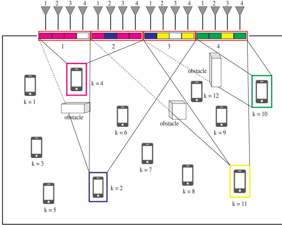
Figure 1.7 – Example of an XL ULA with four SAs, each with four antennas. UEs have different VRs and consequently distinct associated SAs and channel gains to establish communication (Nishimura et al., 2020).
