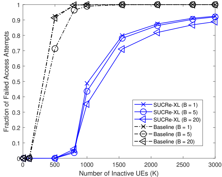
Figure A.7 – Probability of failed access attempt vs. the number of iUEs ( K ), for the SUCRe-XL and Baseline protocols for different numbers of subarrays ( B ), considering the uncorrelated Rayleigh fading model ( P_b = 0.5 ).
