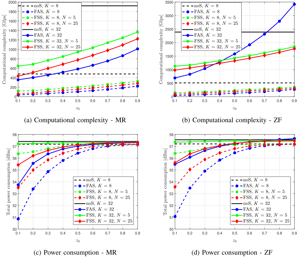
Fig. 4. Computational complexity and power consumption with FSS and FAS antenna selection schemes and MR or ZF combiners.
