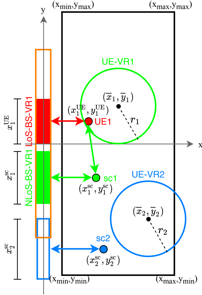
Figure 2.3 – Simplified example of a XL-MIMO system, with 1 user and two scatterers. The user sees a portion of the array through a LoS propagation and other portion of the linear array through a NLoS propagation via scatterer sc1.
