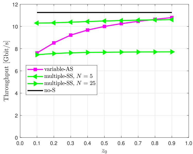
Figure 4.8 – Comparison among no-S, variable-AS and multiple-SS, regarding the throughput, as a function of the parameter z_0 of the algorithms 3.2 and 3.3; K = 32 ; ZF combiner.
