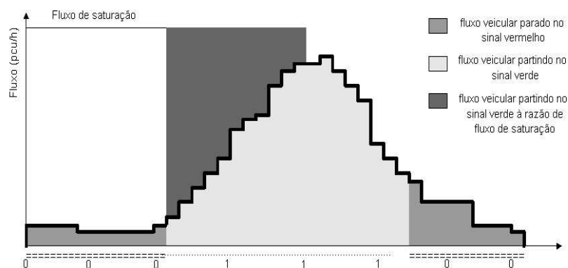
Figura 2.5 – Perfil IN-profile
