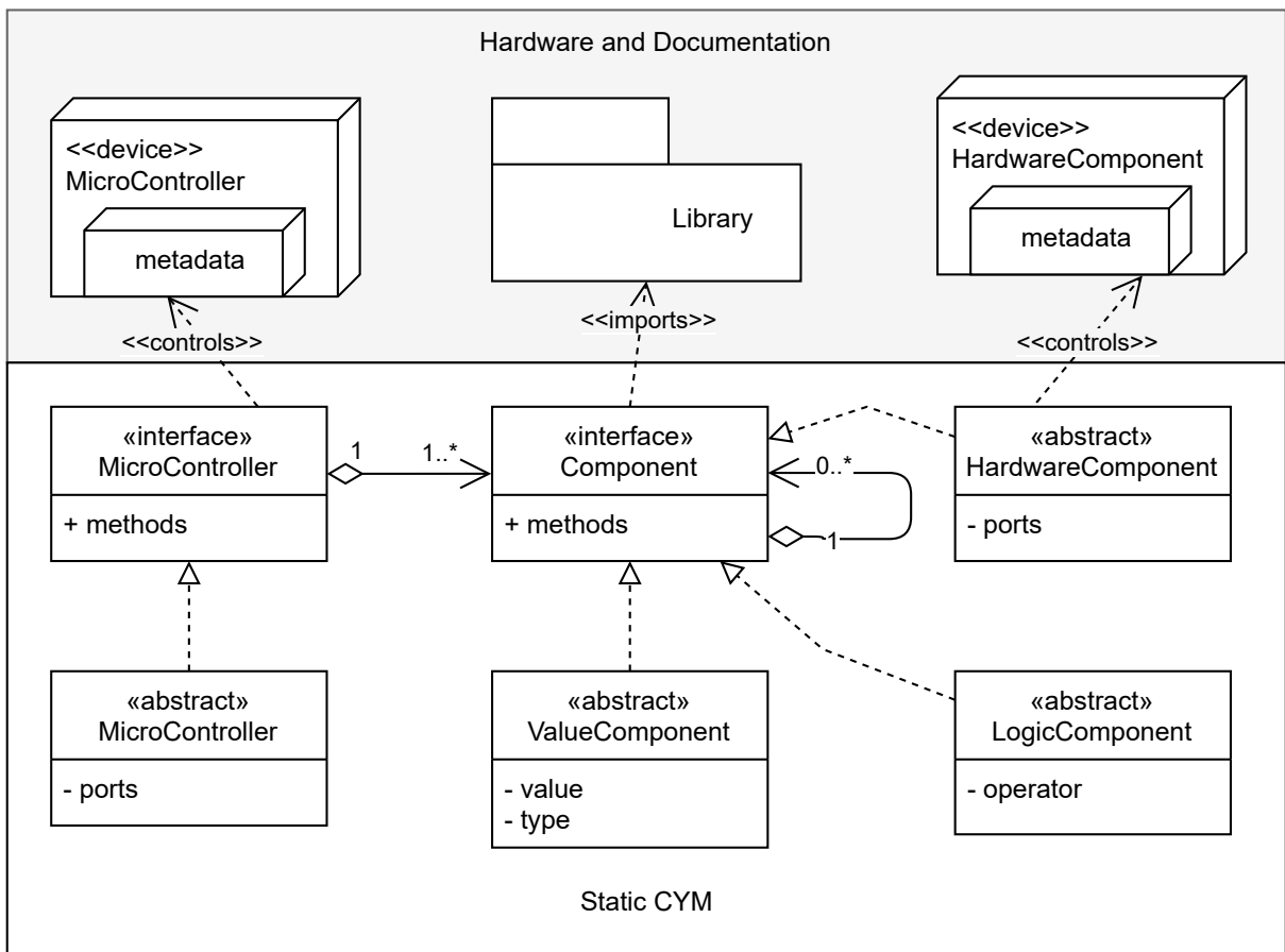
Figure 11 – The hardware-based static CYM.
