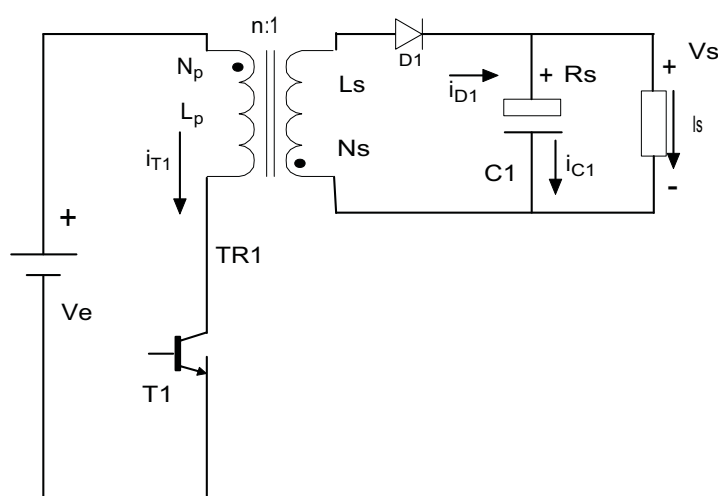
Figura 23 – Conversor Flyback.
